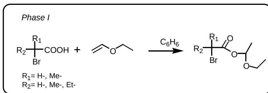
Scheme 1. Synthesis of \alpha -bromo esters-acetals (Phase I)
