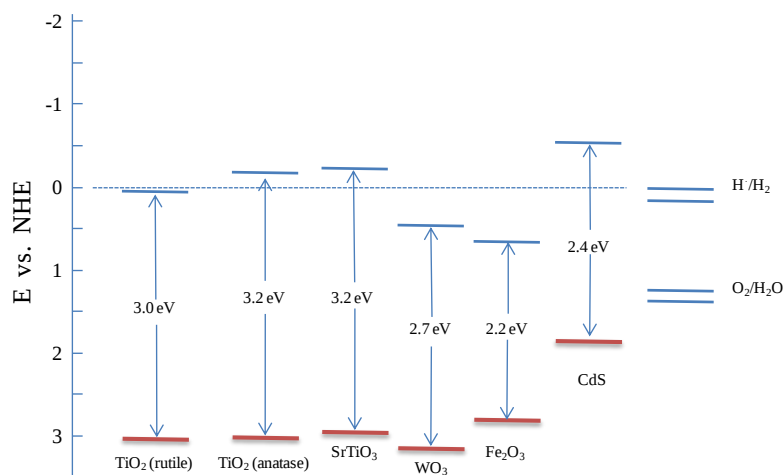
Figure 2. Valence and conductance band positions for various semiconductors and useful, relevant redox couples at \text{pH} \approx 0 . In order to photoreduce a chemical species, the conductance band of the semiconductor must be more negative than the reduction potential of the chemical species; to photo-oxidize a chemical species, the potential of the valence band of the semiconductor must be more positive than the oxidation potential of the chemical species.
