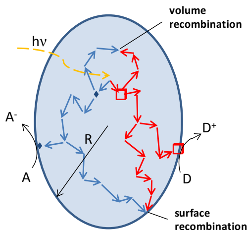
Figure 3. Fate of electrons and holes within a spherical particle of titania in the presence of acceptor (A) and donor (D) molecules
