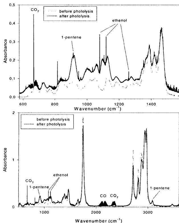
Fig. 1 FTIR spectrum of 100 mTorr n -heptanal, before and after photolysis (6 TL/12 lamps, 100 Torr synthetic air). Major products, CO, pent-1-ene, and ethenol, and CO 2 which is formed as a by-product, are marked (exact positions of the peaks are given in the main text).
