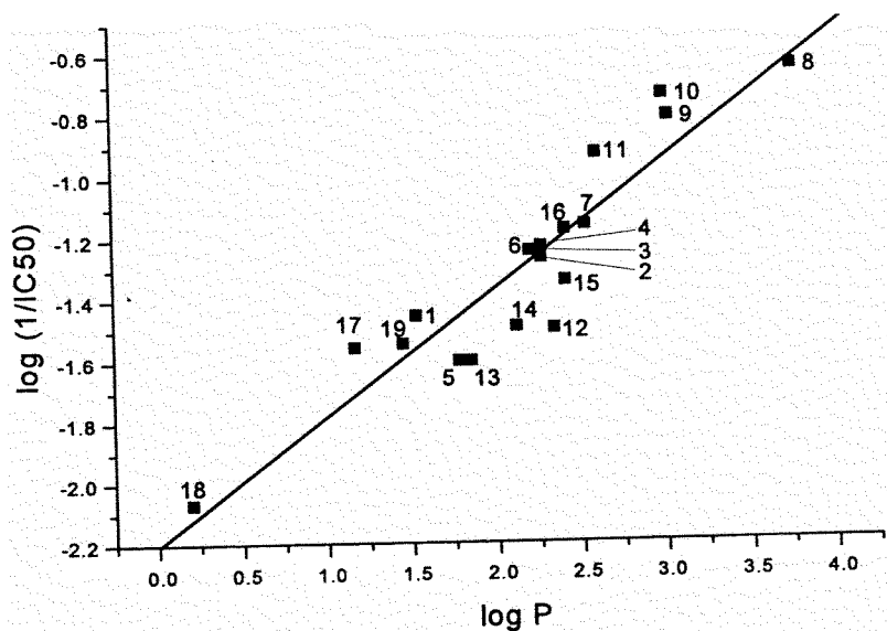
Fig. 1. Correlation between the lipophilicity constant ( \log P ) and -\log (1/\text{IC}_{50}) .
