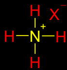
AMONIUM JON
