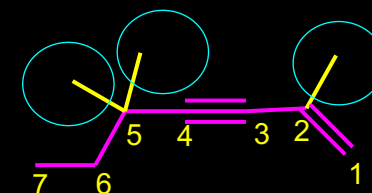
AutoNom Name: 2,5,5-Trimethyl-hept-1-en-3-yne
