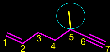
AutoNom Name: 5-Methyl-hept-1-en-6-yne
