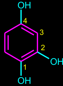
BENZEN-1,2,4-TRIOL
