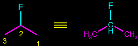
2-FLUOR-PROPAN
