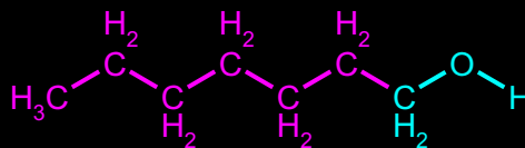
Heptan-1-ol
