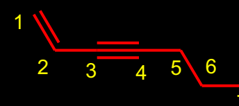
AutoNom Name: Hept-1-en-3-yne
