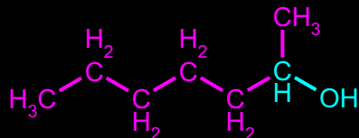
Heptan-2-ol
