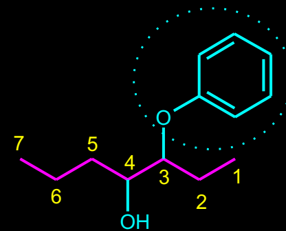
3-Fenoksi-heptan-4-ol
