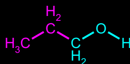
Propan-1-ol
