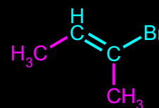
AutoNom Name: (E)-2-Bromo-but-2-ene
