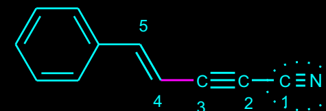
(E)-5-FENIL-PENT-4-EN-2-IN- NITRIL
