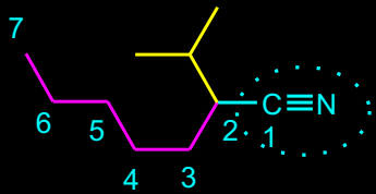
2-izo-PROPIL-HEPTAN-NITRIL
