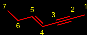
AutoNom Name: (E)-Hept-4-en-2-yne
