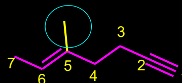
AutoNom Name: (E)-5-Methyl-hept-5-en-1-yne
