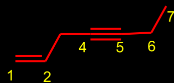
AutoNom Name: Hept-1-en-4-yne
