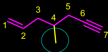
AutoNom Name: 4-Methyl-hept-1-en-6-yne
