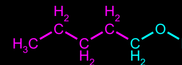
Pentan-1-ol
