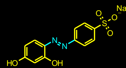
Chrysoine resorcinol
