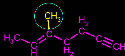
5-METIL-HEPT-5-EN-1-IN
