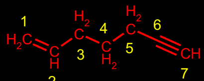
HEPT-1-EN-6-IN
