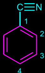
BENZONITRIL
