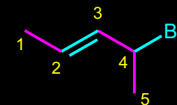
(E)-4-BROM- PENT-2-EN
