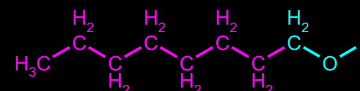
Octan-1-ol
